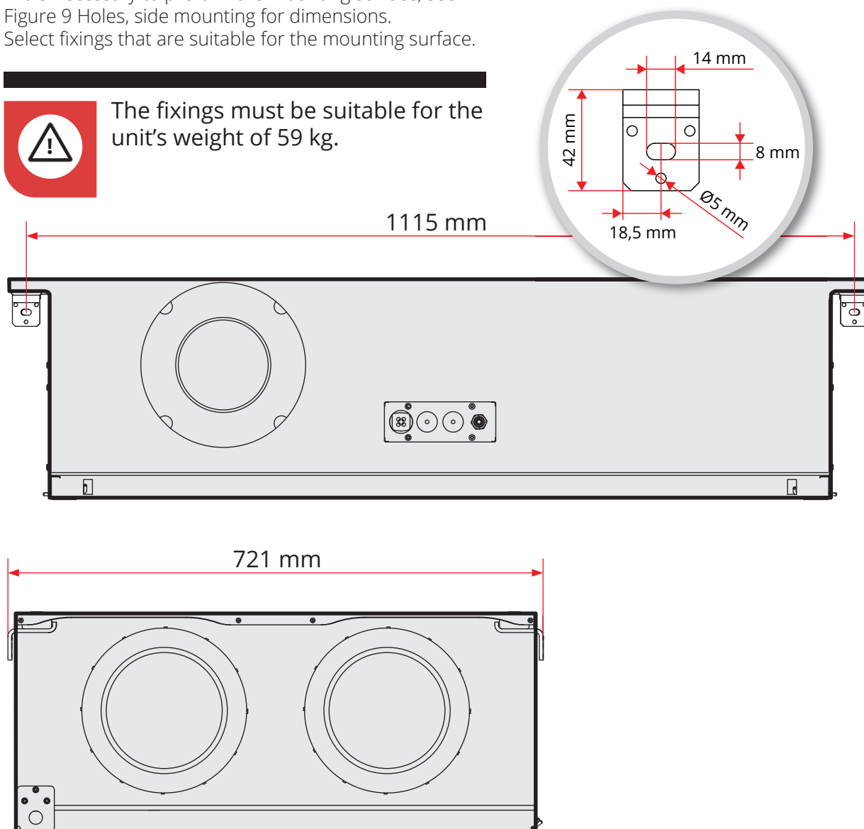
Figure 9 Holes, side mounting
