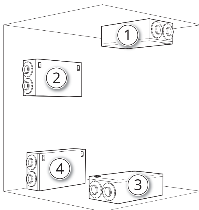
Figure 2 Location options
