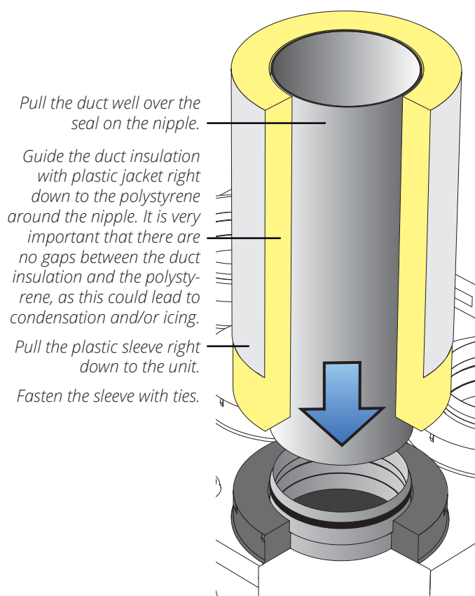
Figure 19 Duct connection
