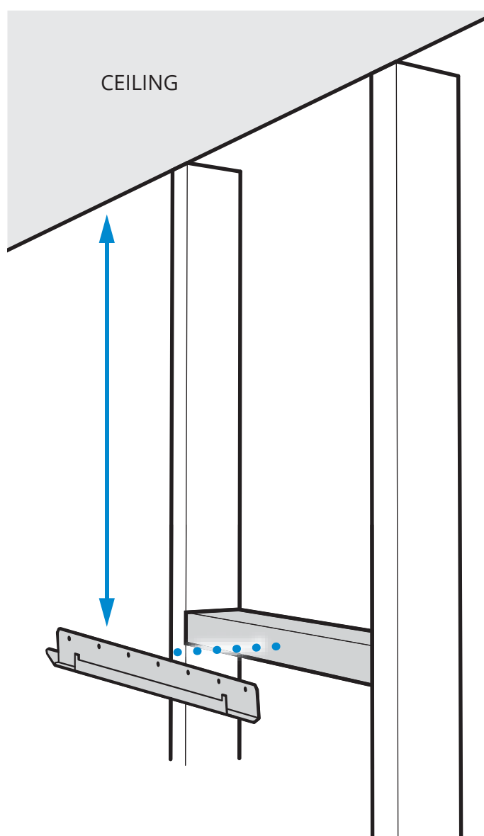
Figure 16 Wall bracket
