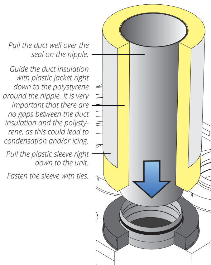
Figure 20 Duct connection
