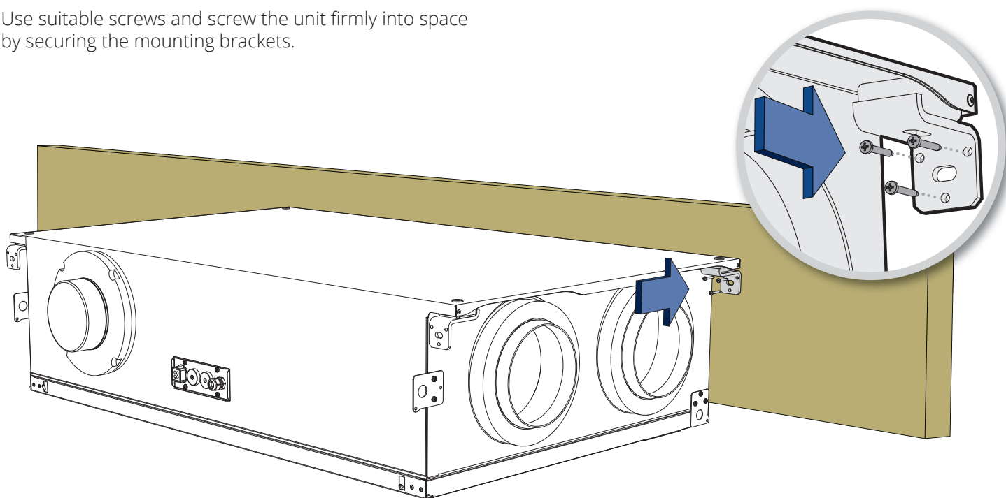
Figure 10 Side mounting
