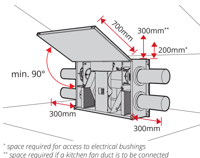
Figur 19 Space requirements for vertical floor mounting
