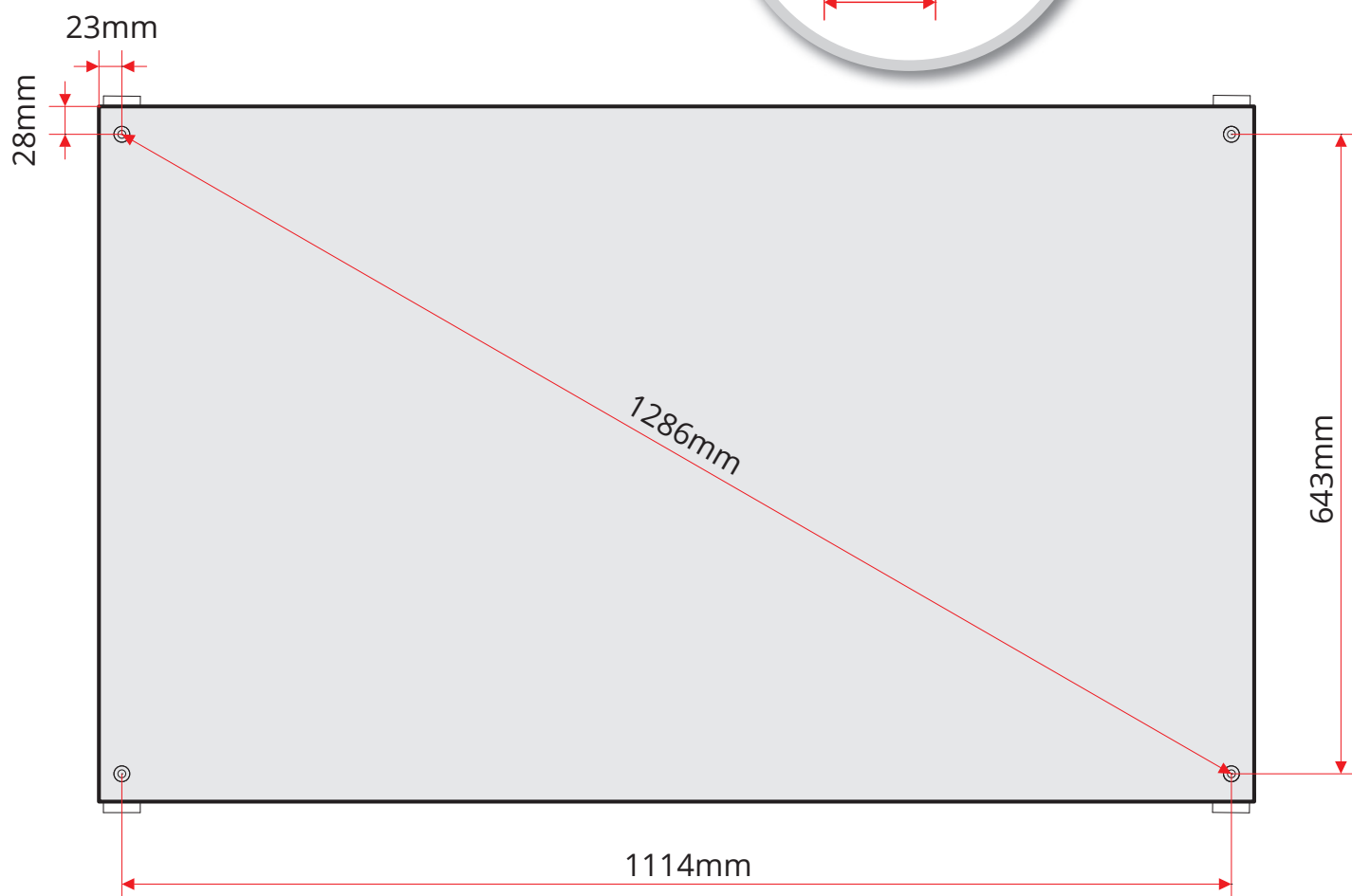
Figure 5 Holes, top mounting
