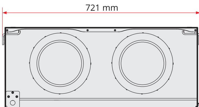
Figure 9 Holes, side mounting
