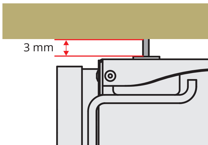
Figure 7 Gap to mounting surface
