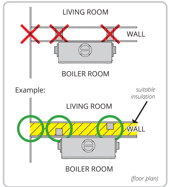
Figure 12 Wall construction
