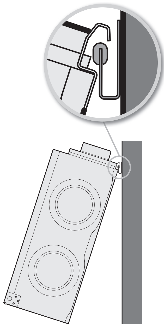
Figure 15 Fitting the wall bracket
