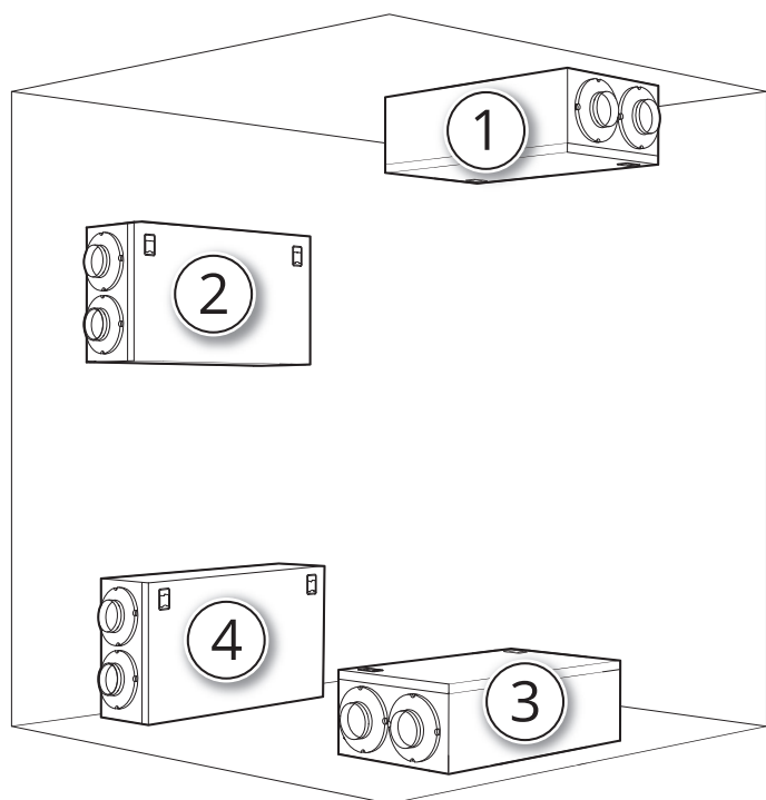
Figure 2 Location options
