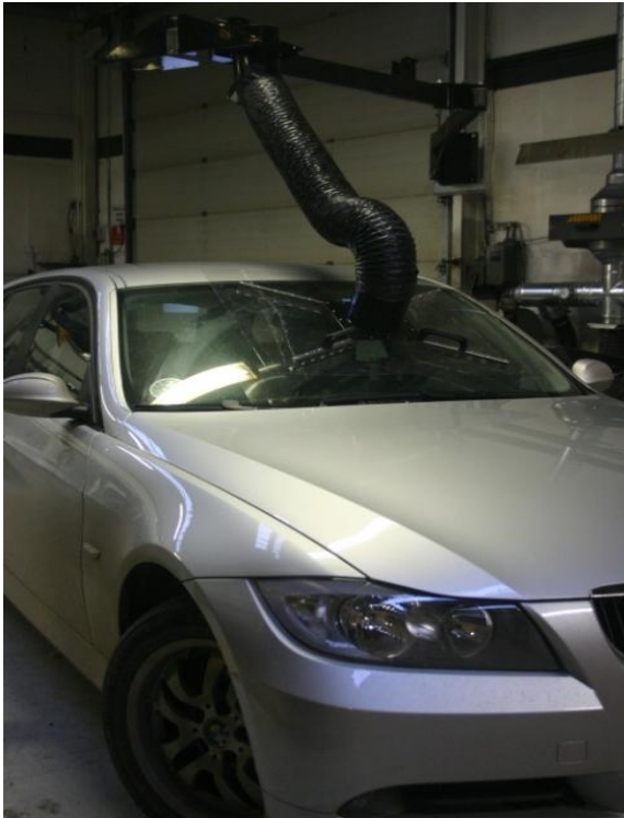
Extraction hood for windscreen gluing in use
