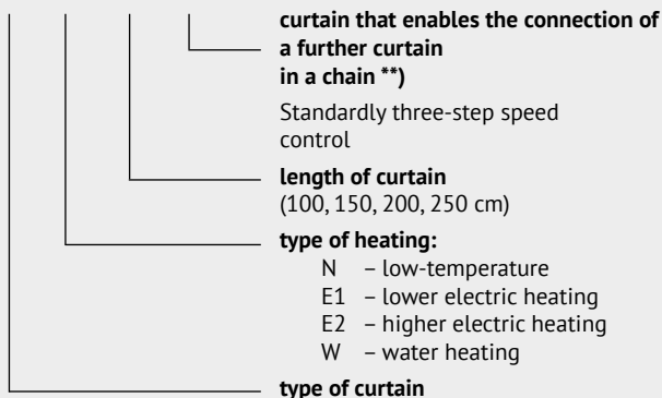
Illustration 10 - D2 air curtains marking
