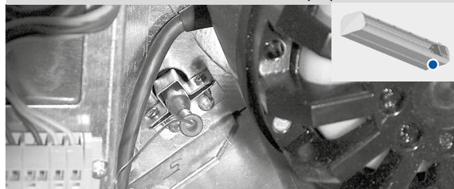
Illustration 17 - thermo-valve's feeler (D2)
