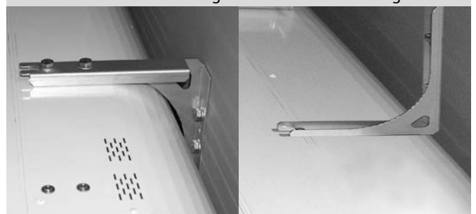
Illustration 19 - mounting console and fastening
