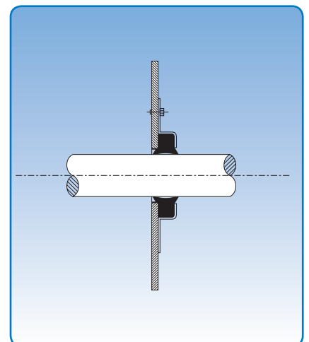
Shaft gasket
