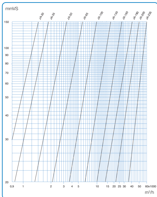
Diagram states pressure loss in cyclone at a given air volume measured in \text{m}^3/\text{h} .
