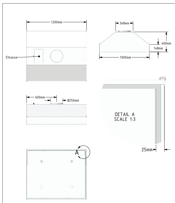
02-210 Hood
