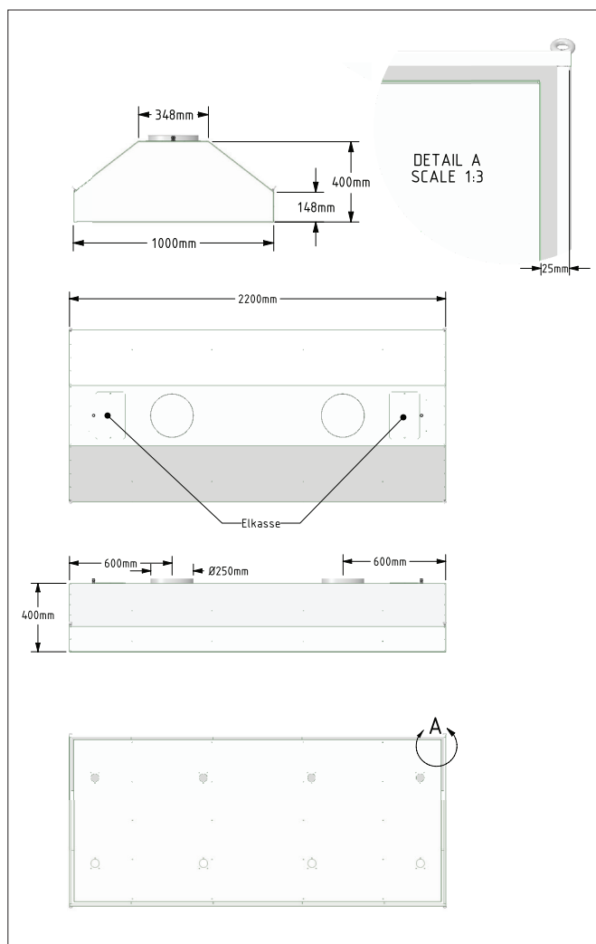
02-211 Hood
