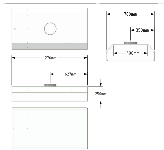
02-212 Hood
