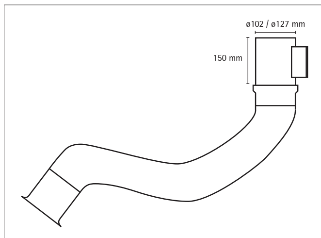
Wall console
