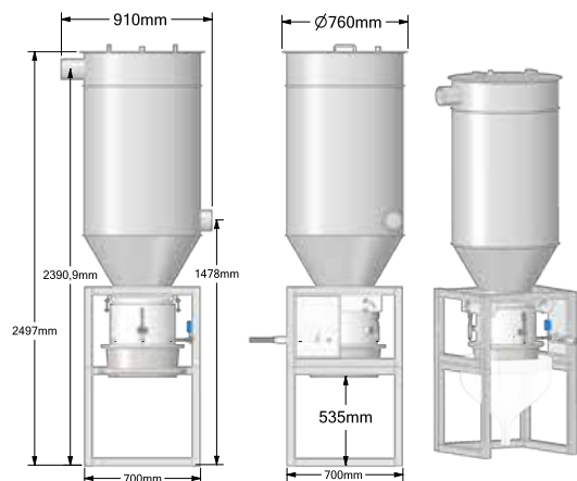
Longopac solution
