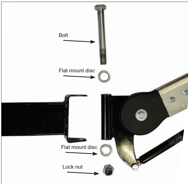
3. Once the wall bracket is installed on the wall, the arm is mounted. At the top of the inner joint the bolt, flat mount disc, and the lock nut is fitted. See image. Tighten as needed.
