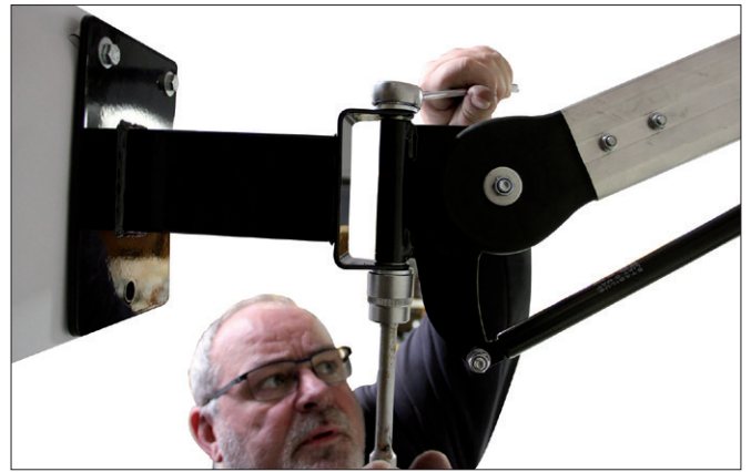
4. Use the correct tool to secure the arm to the wall bracket. Tighten as needed.
